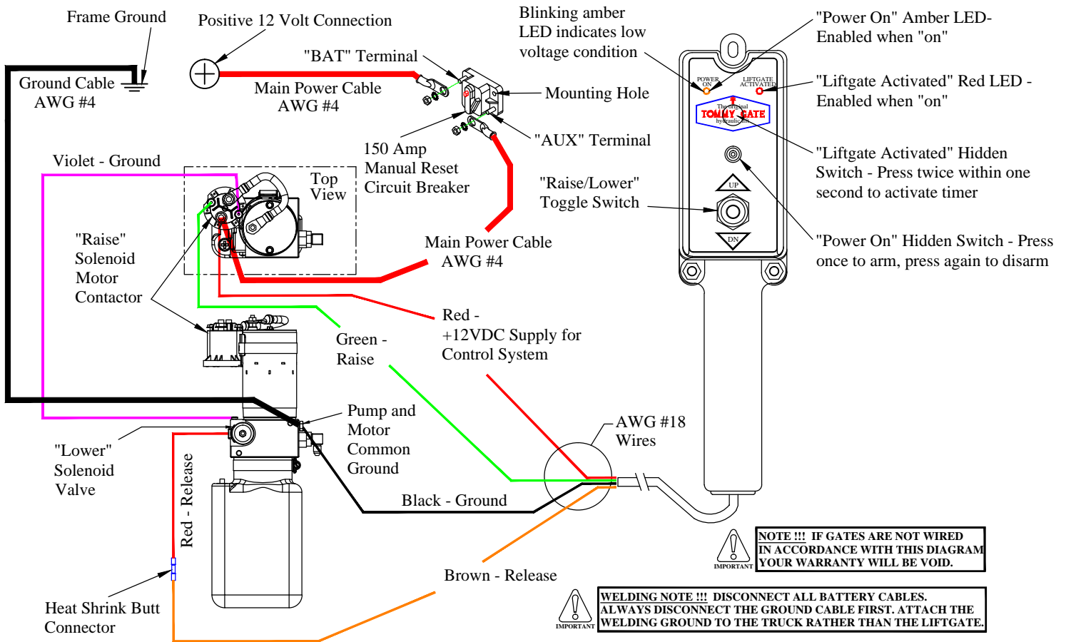
Figure 21: Wiring Diagram.
