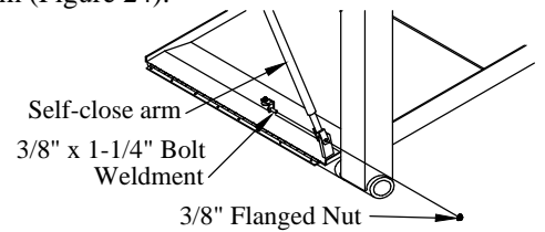
Figure 24: Self-close arm parts.
