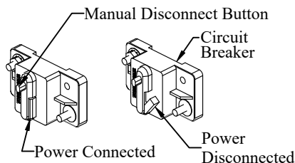
Figure 2: Circuit Breaker
