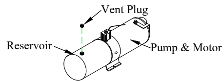
Figure 16: Vent plug.
