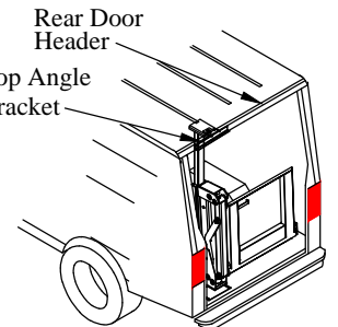
Figure 9: Liftgate in rear opening.
