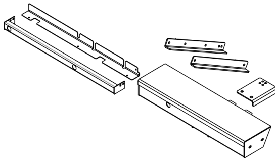
Sensor Bar*
