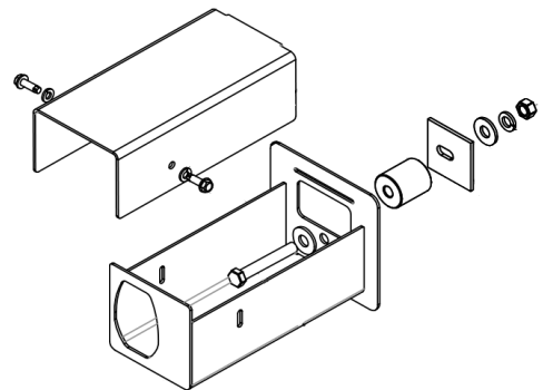
Camera Housing*
