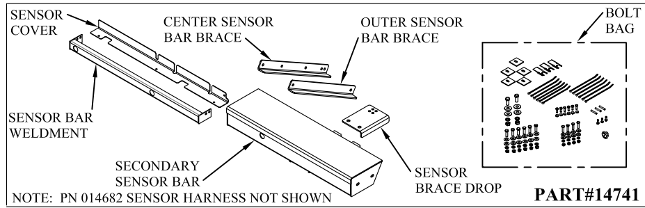
Figure 1: TRANSIT SENSOR KIT PART IDENTIFICATION.
