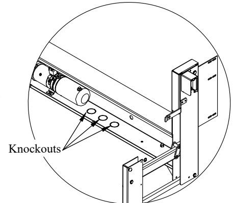
Figure 10: Knockout hole location.
