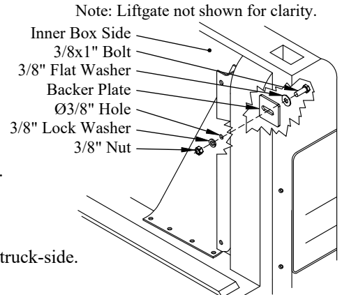
Figure 13: Additional support location.
