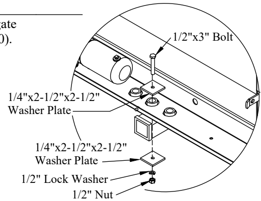
Figure 20: Lower bracket support (Class 4 hitch).
