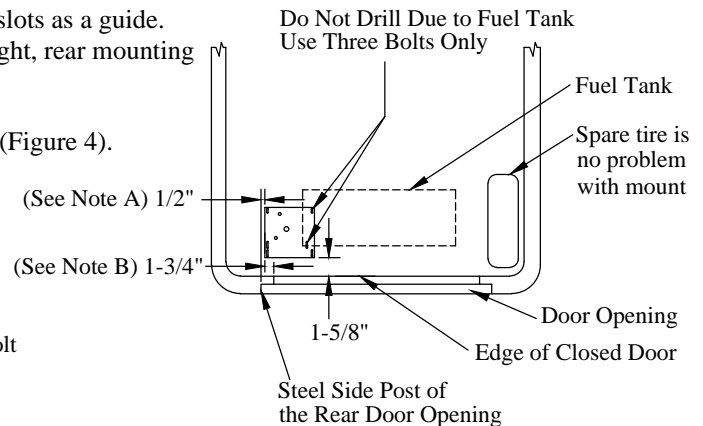
Figure 3: Base plate location and obstructions.
