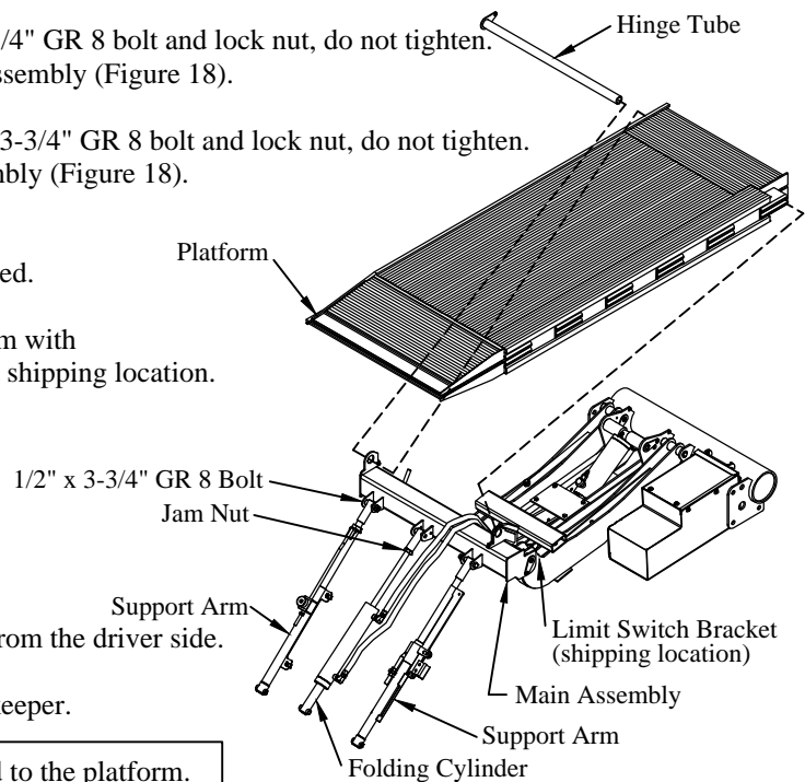
Figure 18: Platform parts location.
