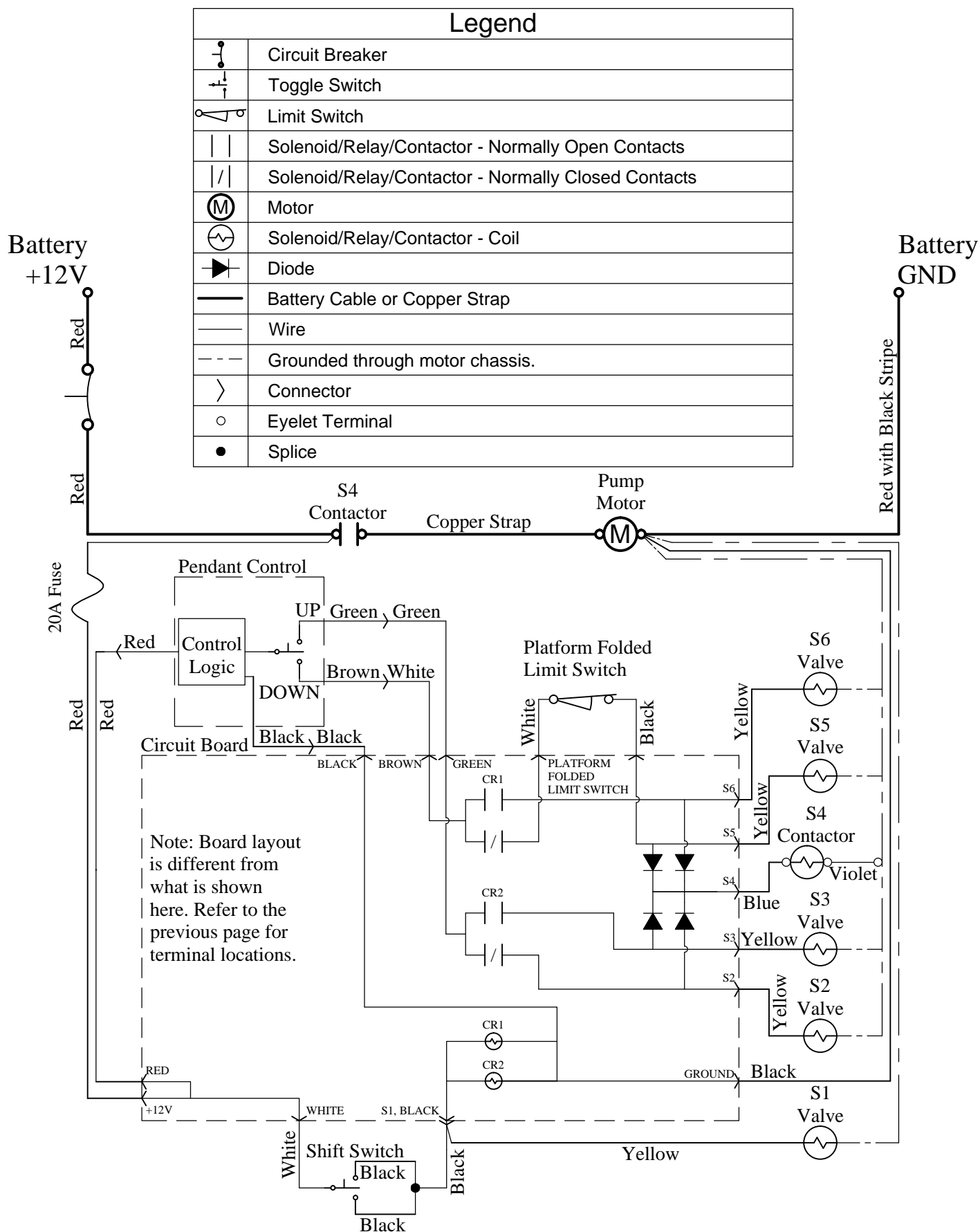
Figure 17: Power unit control circuit.
