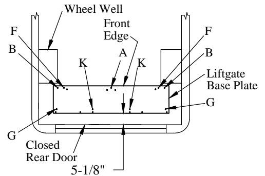
Figure 10: Bolt locations (top view).
