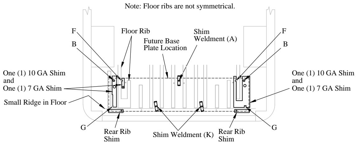
Figure 7: Rib shim locations (top view).
