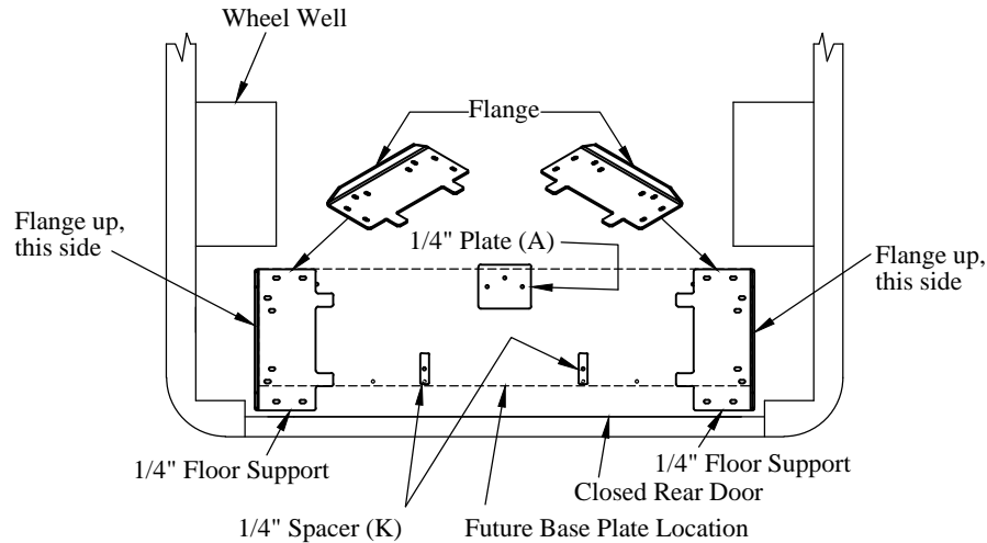
Figure 8: Floor support locations (top view).
