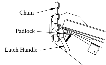
Figure 21: Chain latch and padlock location.
