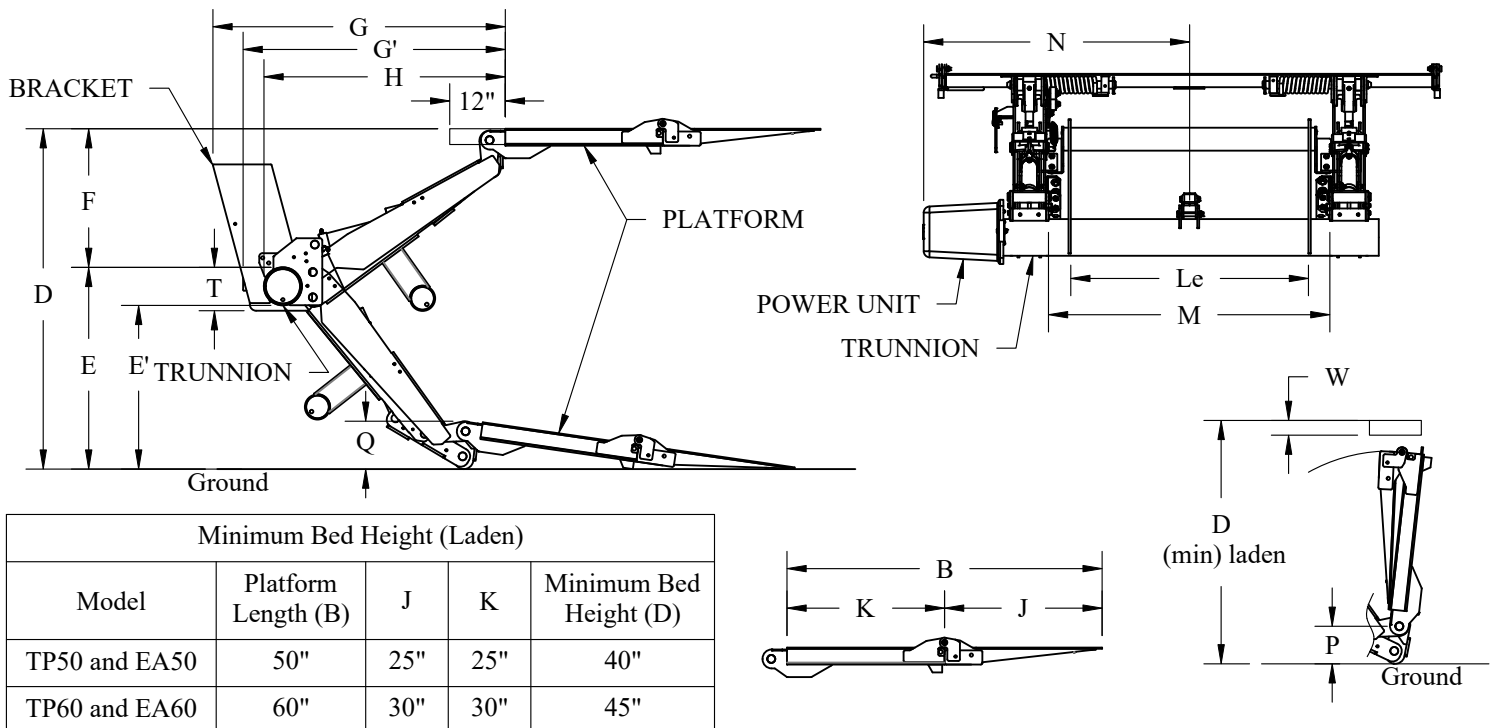
Figure 2: Liftgate General Dimensions
