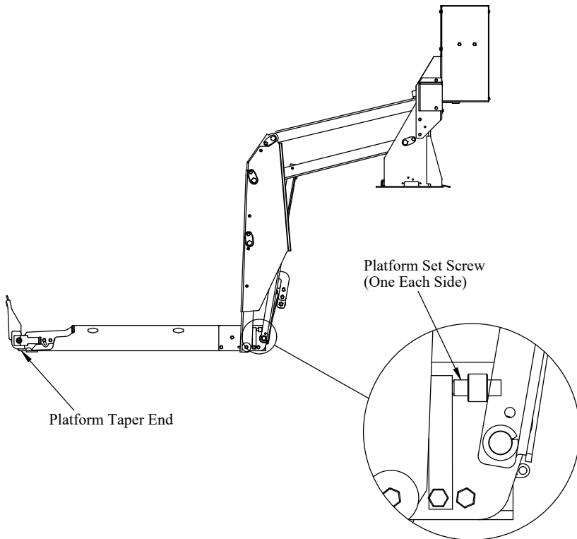
Figure 7: Platform.
