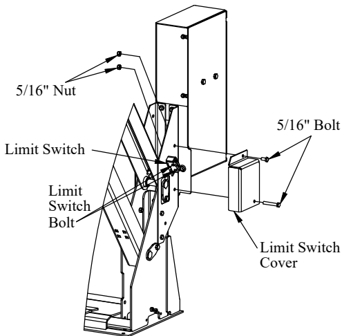
Figure 6: Limit Switch.
