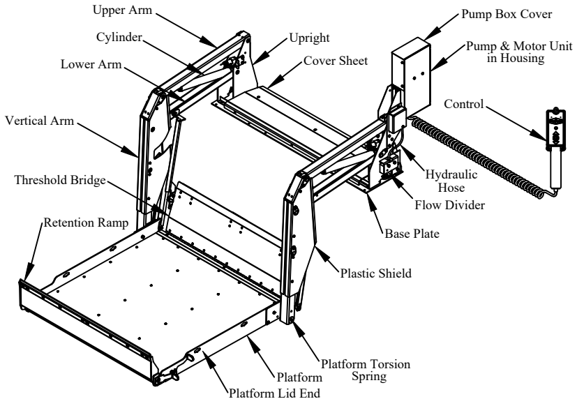
Figure 1: Parts identification.
