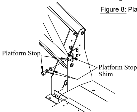
Figure 9: Platform stops.
