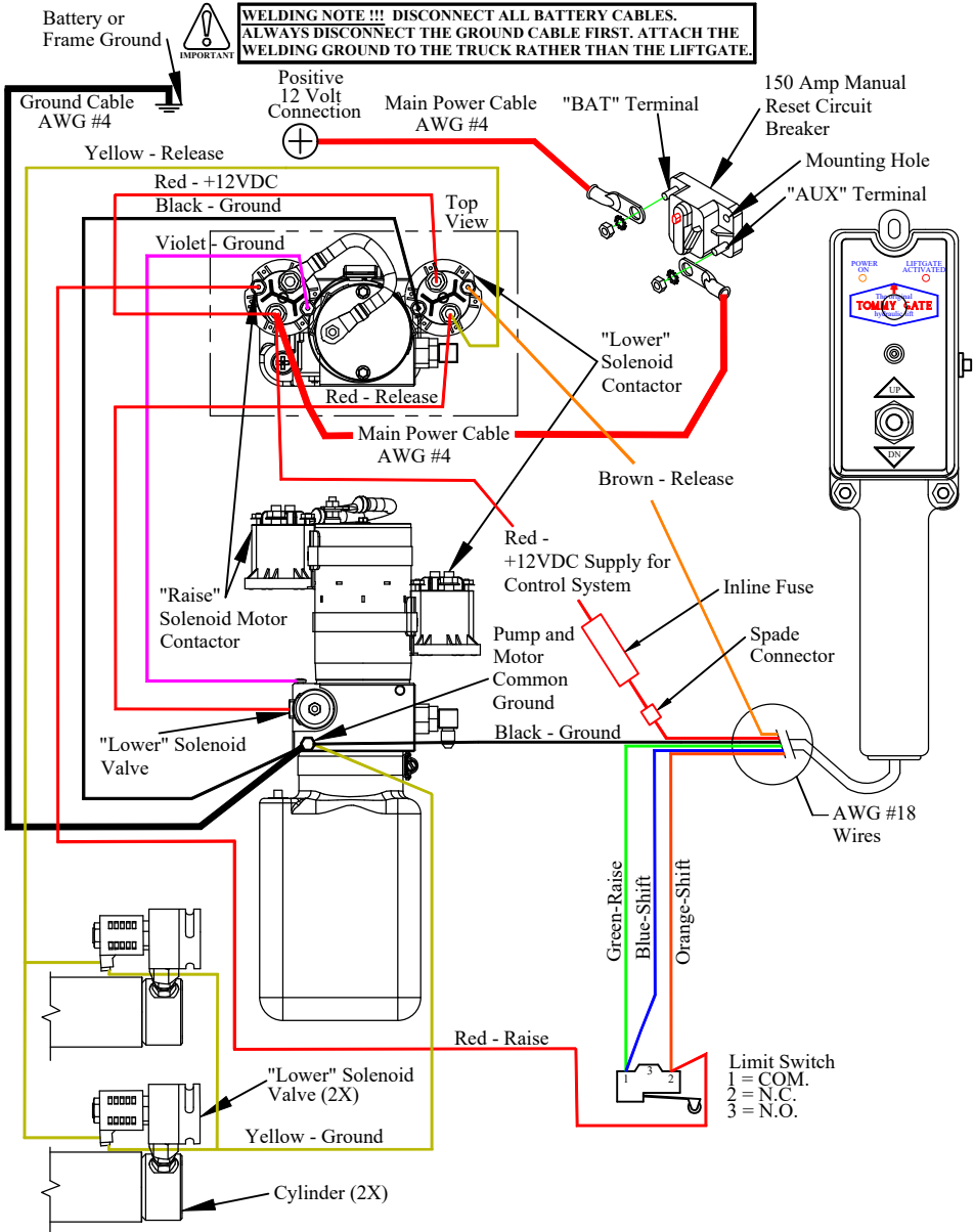
Figure 5: Wiring diagram.
