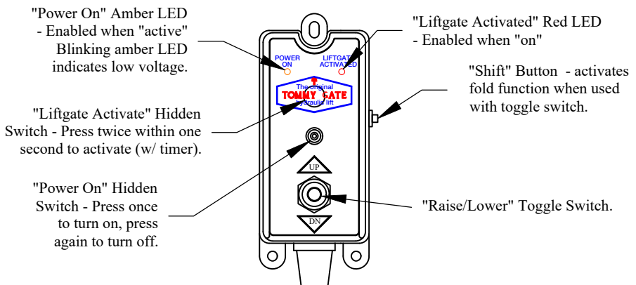
Figure 2: Control.
