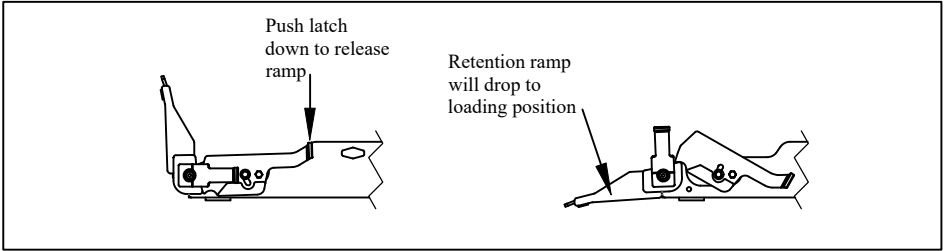
Figure 3: Loading position.
