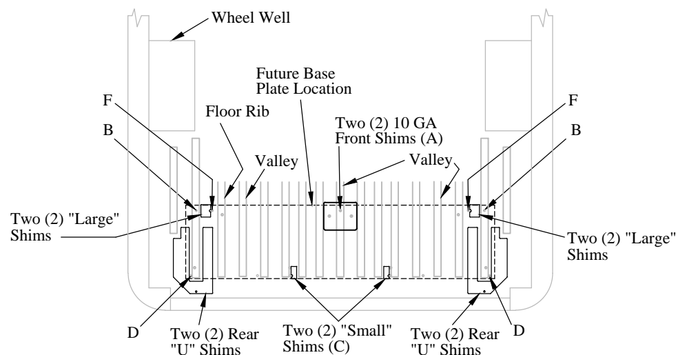
Figure 7: Rib shim locations (top view).
