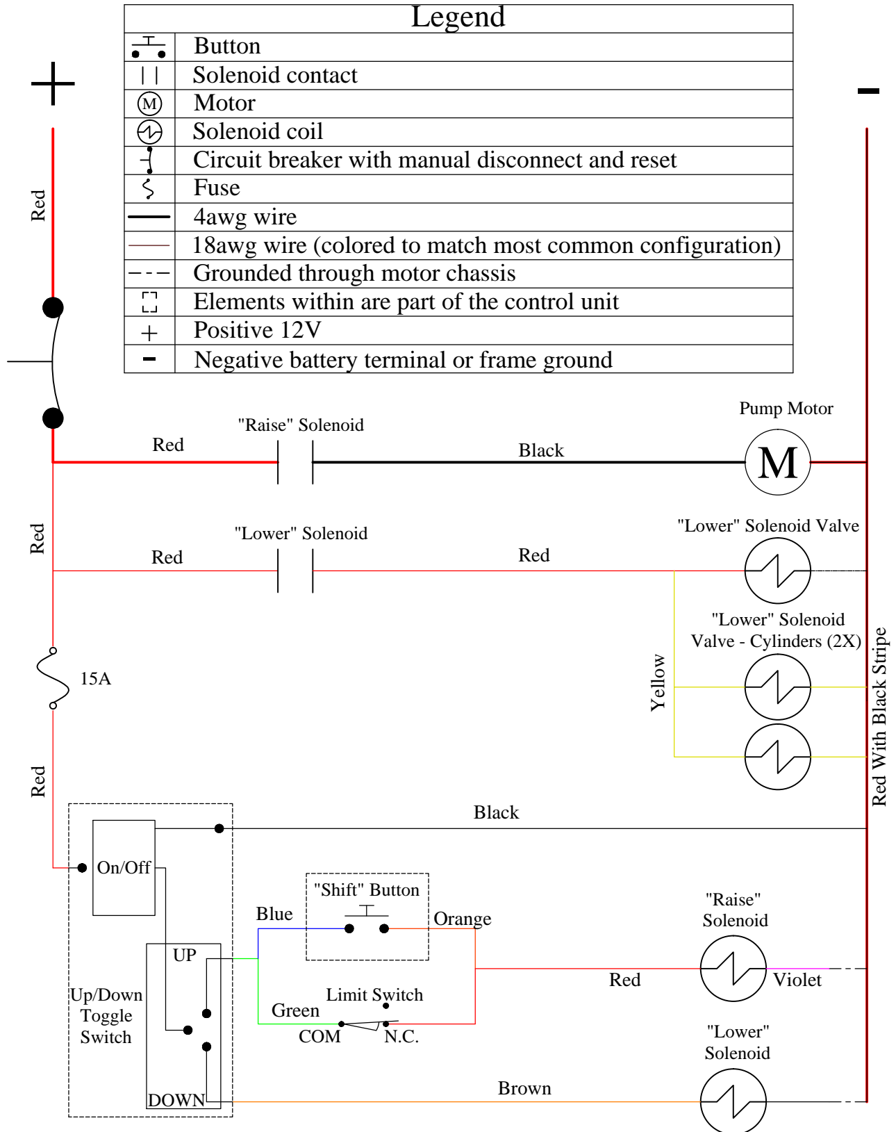
Figure 17: Power unit control circuit.
