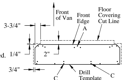
Figure 5: Floor covering cut location (top view).
