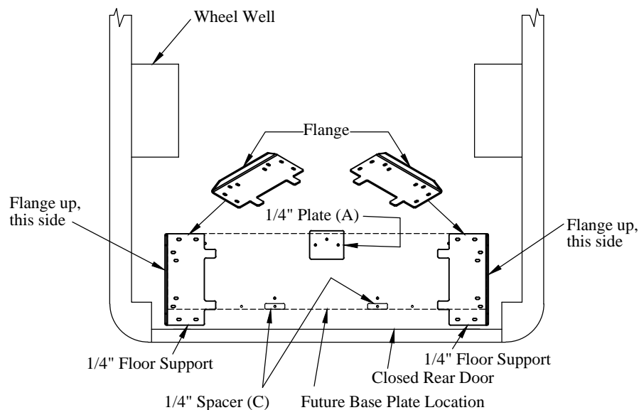
Figure 8 : Floor support locations (top view).
