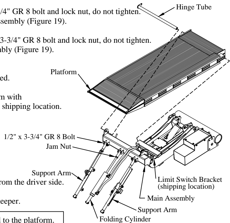
Figure 19: Platform parts location.
