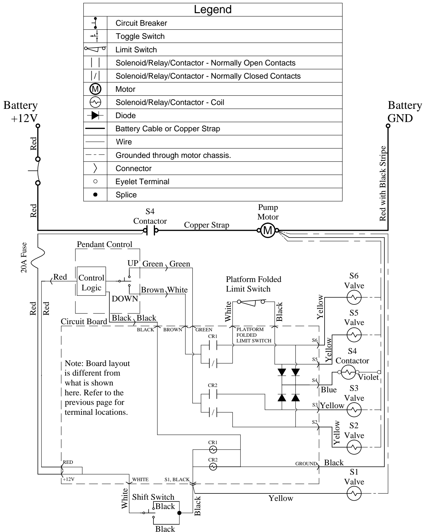
Figure 18: Power unit control circuit.
