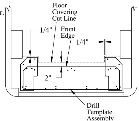
Figure 6: Floor covering cut location (top view).
