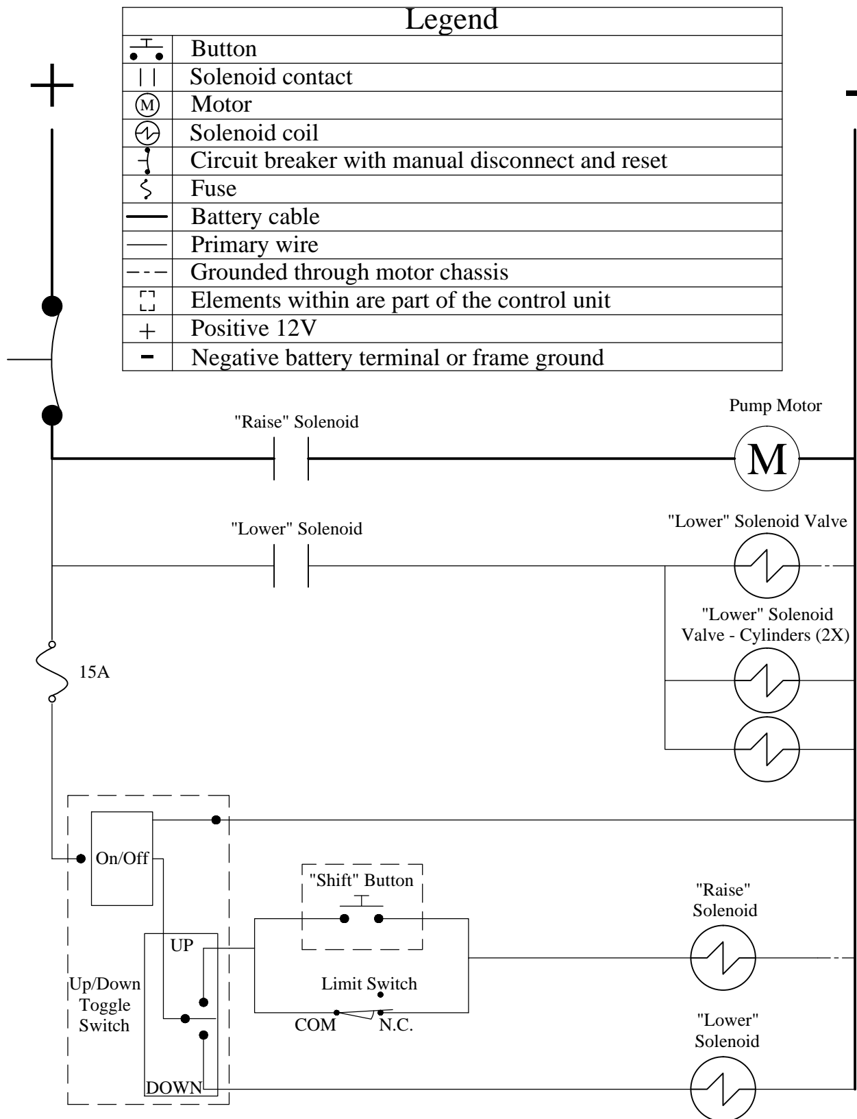
Figure 21 : Power unit control circuit.
