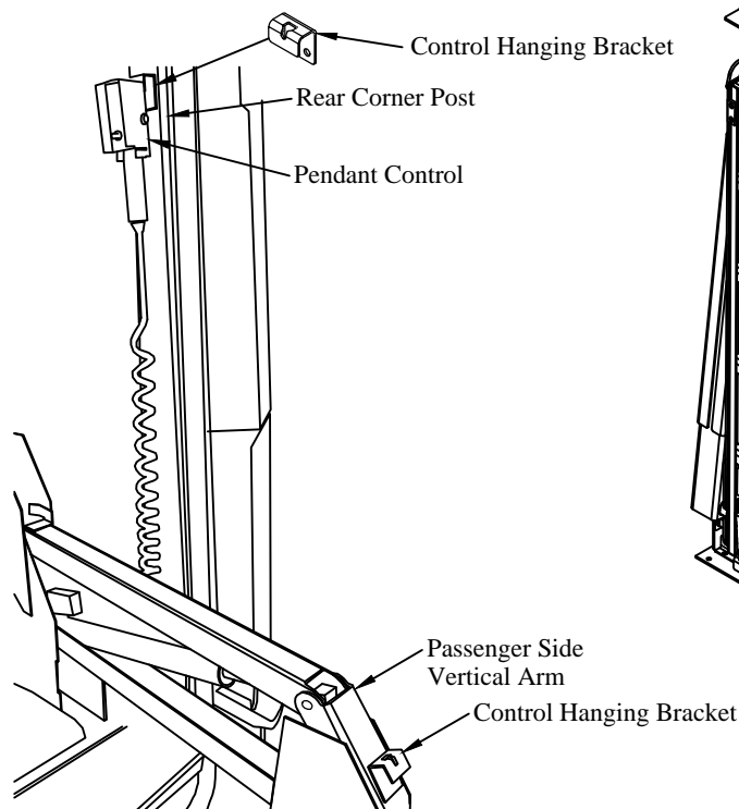
Figure 23: Control Hanging Brackets.
