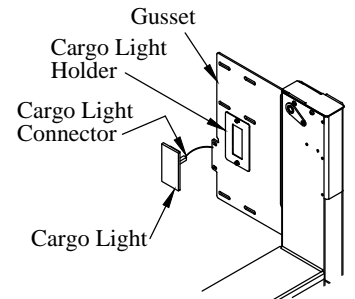
Figure 16: Cargo light.
