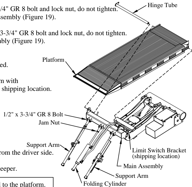
Figure 19: Platform parts location.
