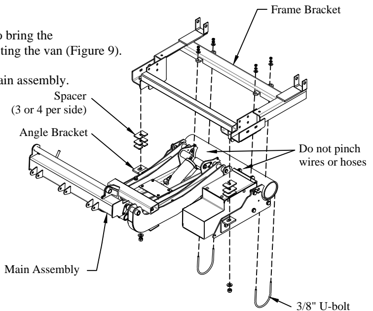
Figure 9: Main assembly position on frame.
