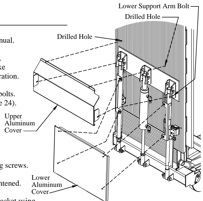
Figure 24: Aluminum cover installation.
