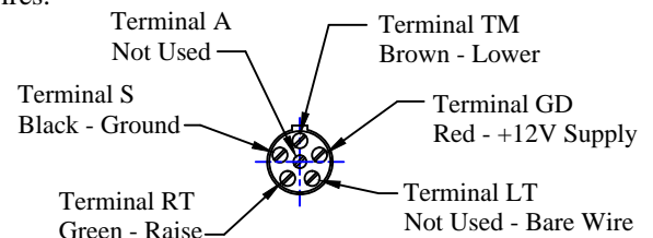
Figure 16: Female connector wiring.
