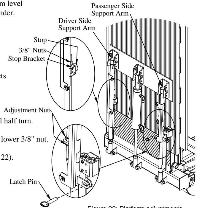
Figure 22: Platform adjustments.
