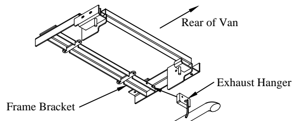
Figure 11: Exhaust hanger location.
