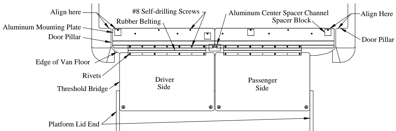
Figure 23: Threshold bridge location.
