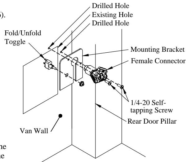
Figure 15: Pendant control female connector location.
