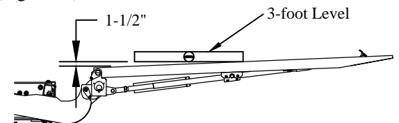
Figure 21: Platform position.
